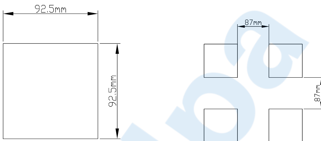
Opening size and minimum distance between square holes of distribution box
